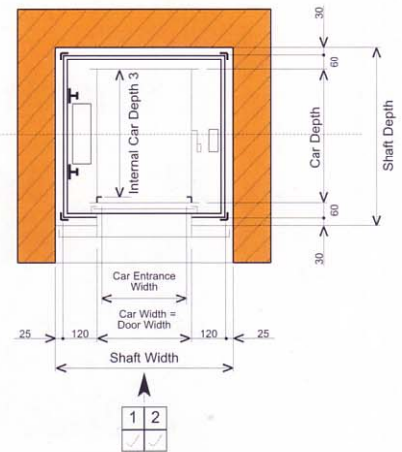
SINGLE ENTRY WITH ROLLER SHUTTER
