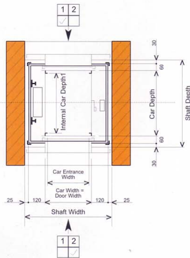
THROUGH ENTRY WITH ROLLER SHUTTERS
