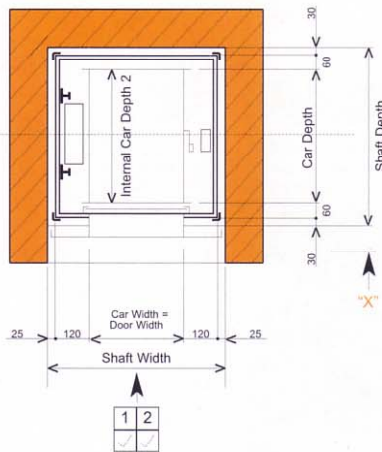
SINGLE ENTRY WITHOUT ROLLER SHUTTER
